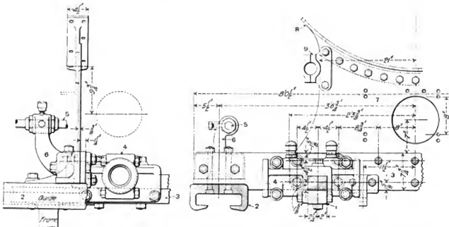
Figs. 1099-1601. Assembled View of Frame Rocker Box and Guide Yoke. Atlantic (4-4-2) Locomotive, Pennsylvania Railroad.
